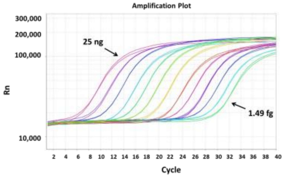
Fig. 1. The amplification plot of real-time PCR with cDNA template ranged from 25 ng to 1.49 fg in quantity, analyzed by using TQ1100 ExcelTaq™ 2X Q-PCR Master Mix (SYBR, no ROX) for qPCR amplification.
